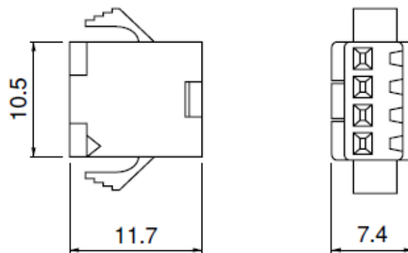
Female Socket
