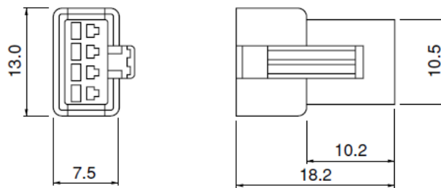
Male Plug
