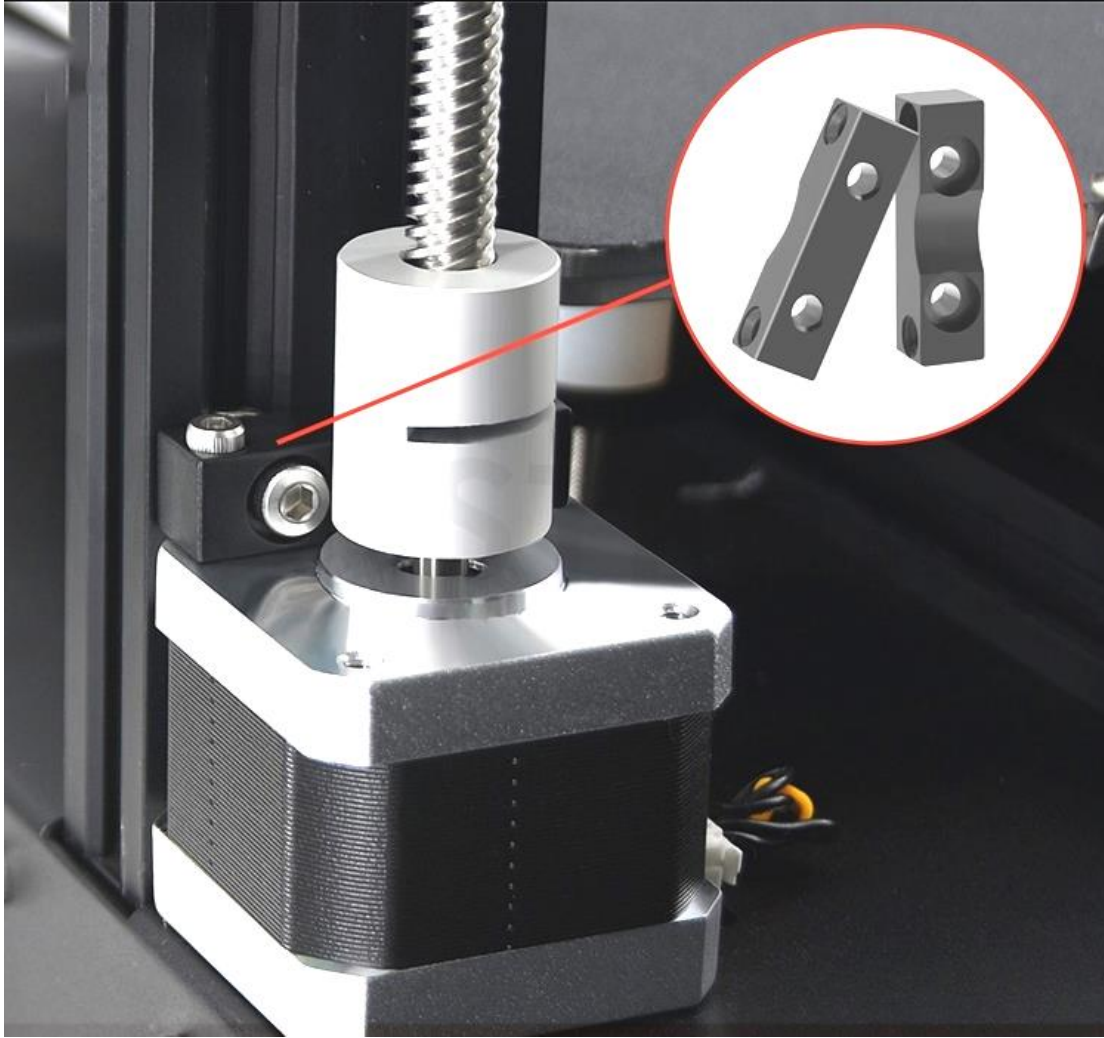
Mounting Z Axis Nema-17 Stepper motor to Aluminum Profile
